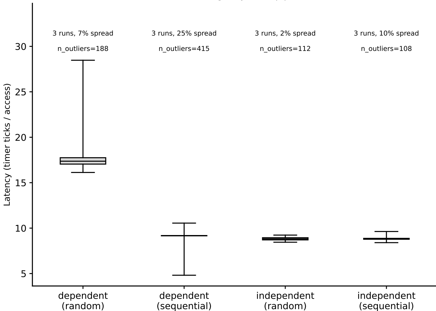
hazel_skylake/phase1_v2: hit-latency box plots, L2 (footprint=1 MiB) (Phase I timing-only, auto pipeline)
