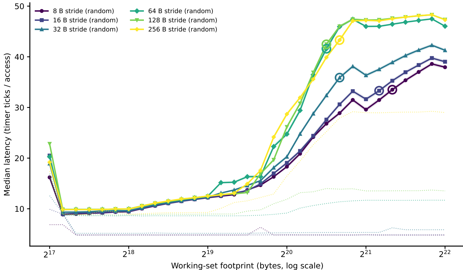
hazel_skylake/phase1_v2: line-size family of curves (dependent pointer chase) (Phase I timing-only, level boundary=1048576B window=[131072,4194304])
