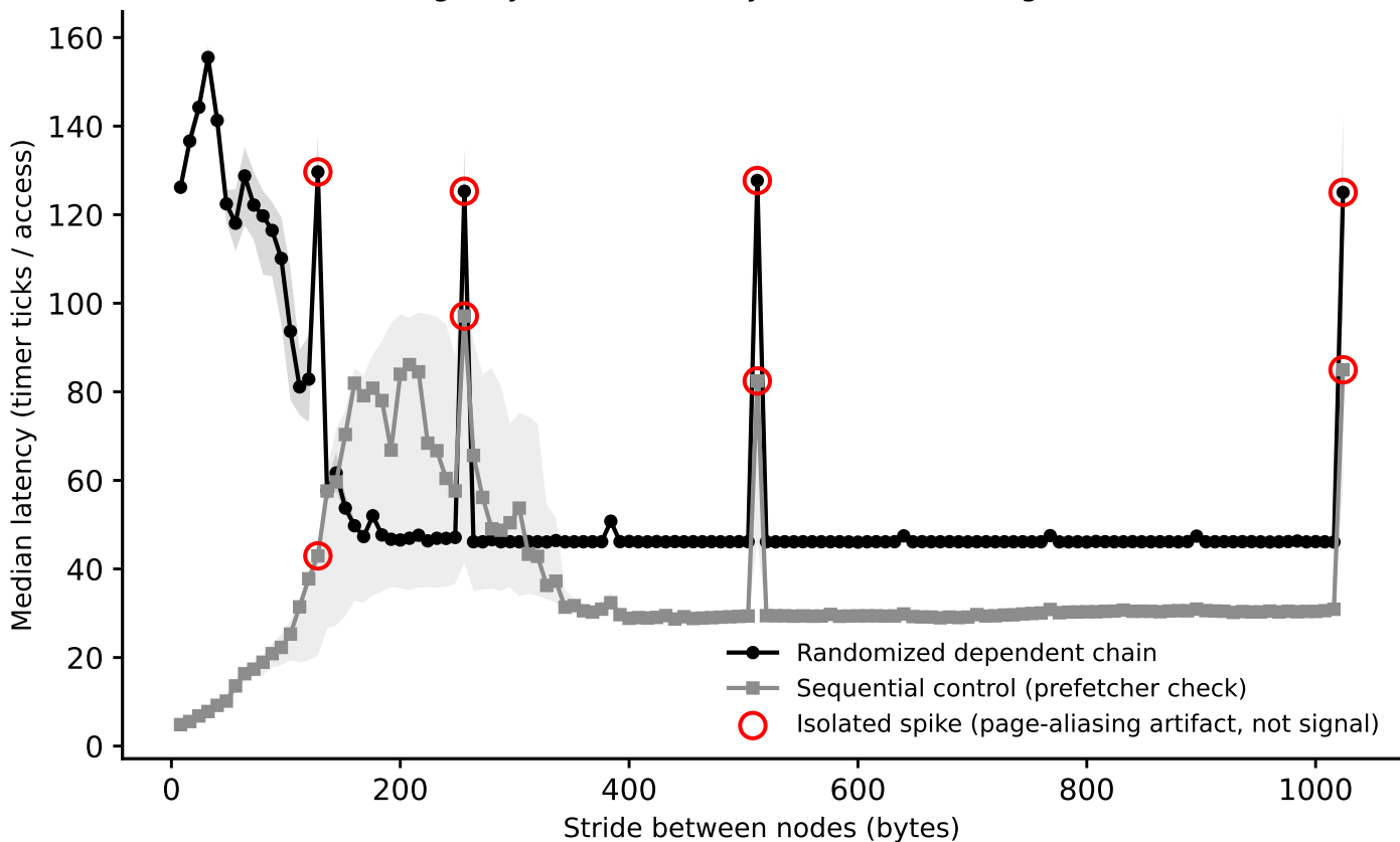
hazel_skylake/phase1_v2: line-size sweep (dependent pointer chase), footprint=45.2548 Mi (Phase I timing-only, level boundary=23726560B, single-curve method)
