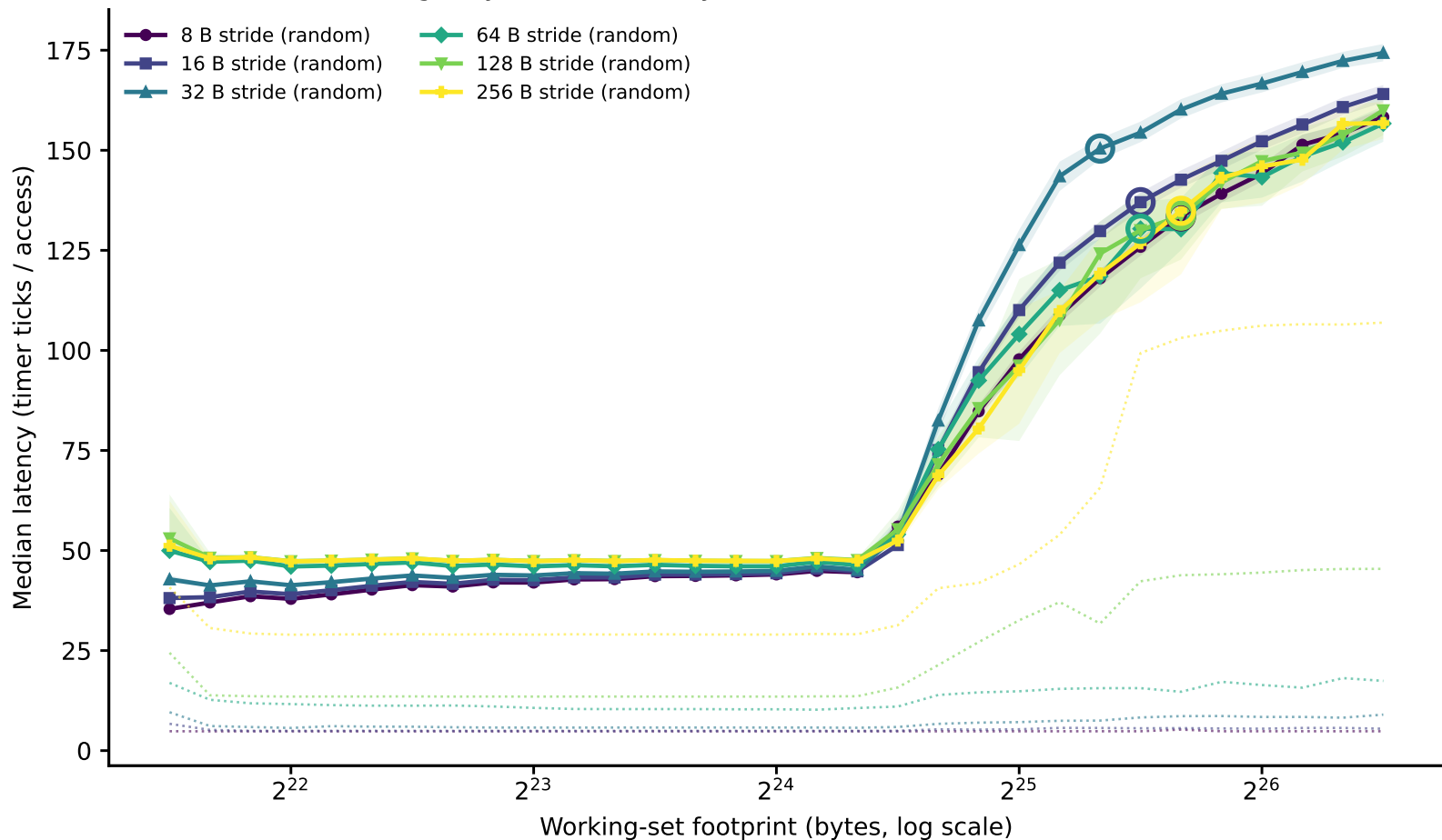
hazel_skylake/phase1_v2: line-size family of curves (dependent pointer chase) (Phase I timing-only, level boundary=23726560B window=[2965820,94906240])
