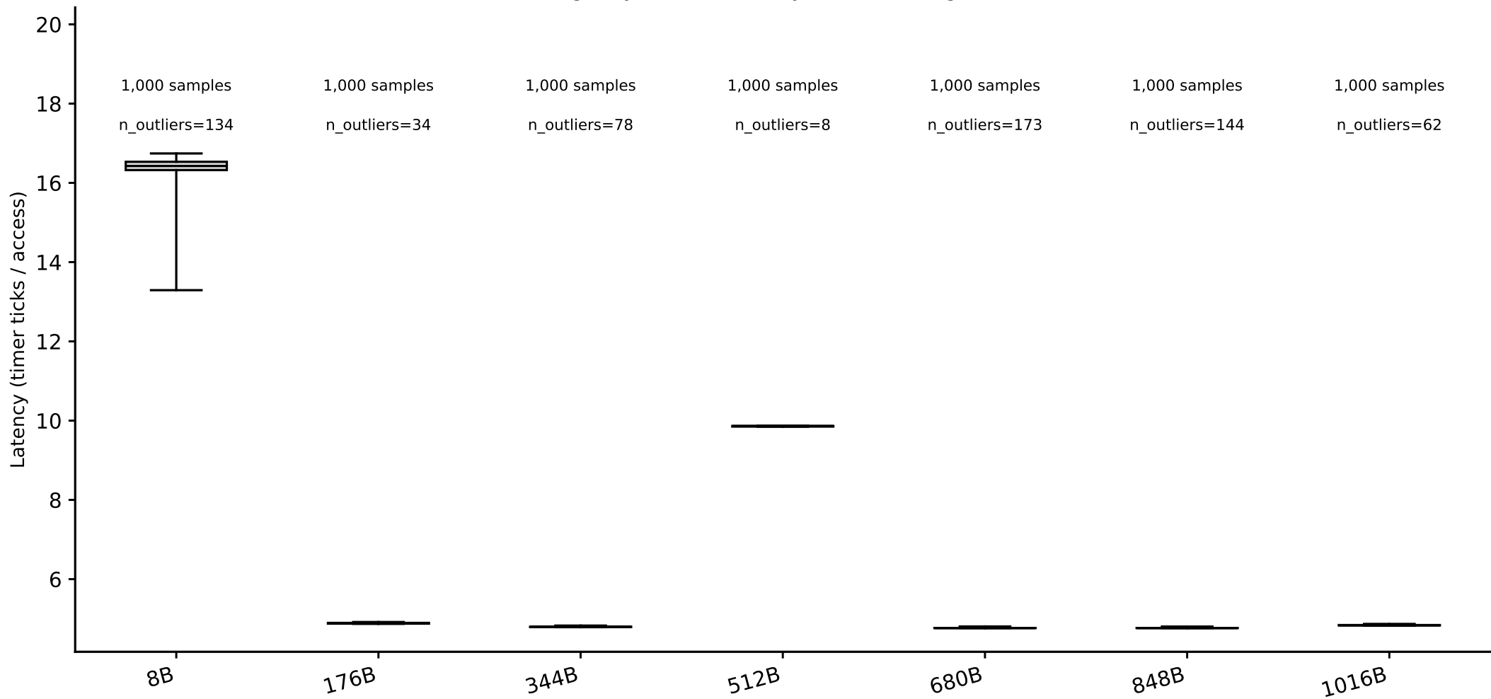
hazel_skylake/phase1_v2: line-size box plots, random pattern (whiskers = p5/p95) (Phase I timing-only, level boundary=32768B, single-curve method)
