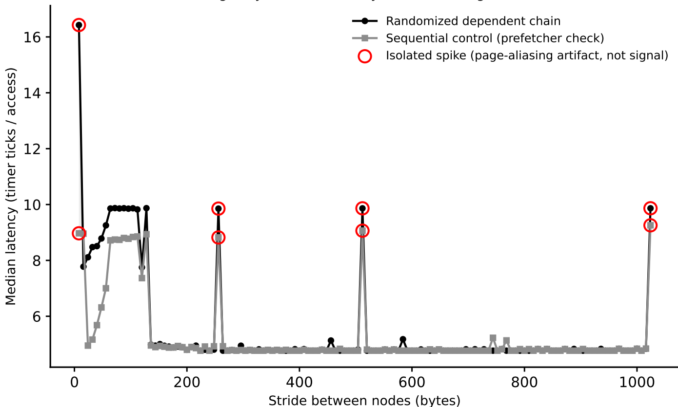
hazel_skylake/phase1_v2: line-size sweep (dependent pointer chase), footprint=64 KiB (Phase I timing-only, level boundary=32768B, single-curve method)
