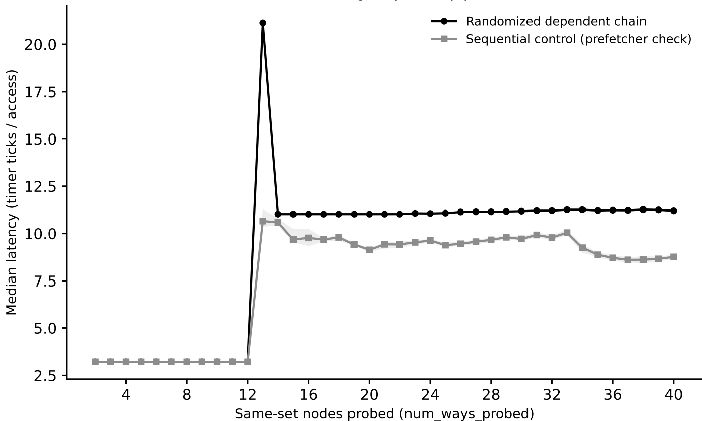
hazel_turin: associativity sweep, L1 (stride=48 KiB) (Phase I timing-only, auto pipeline)
