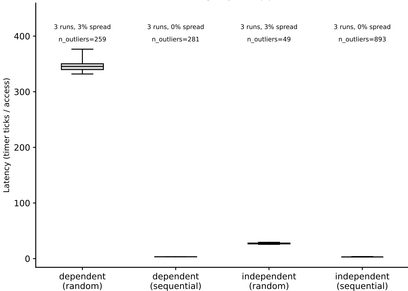
hazel_turin: hit-latency box plots, DRAM (footprint=512 MiB) (Phase I timing-only, auto pipeline)
