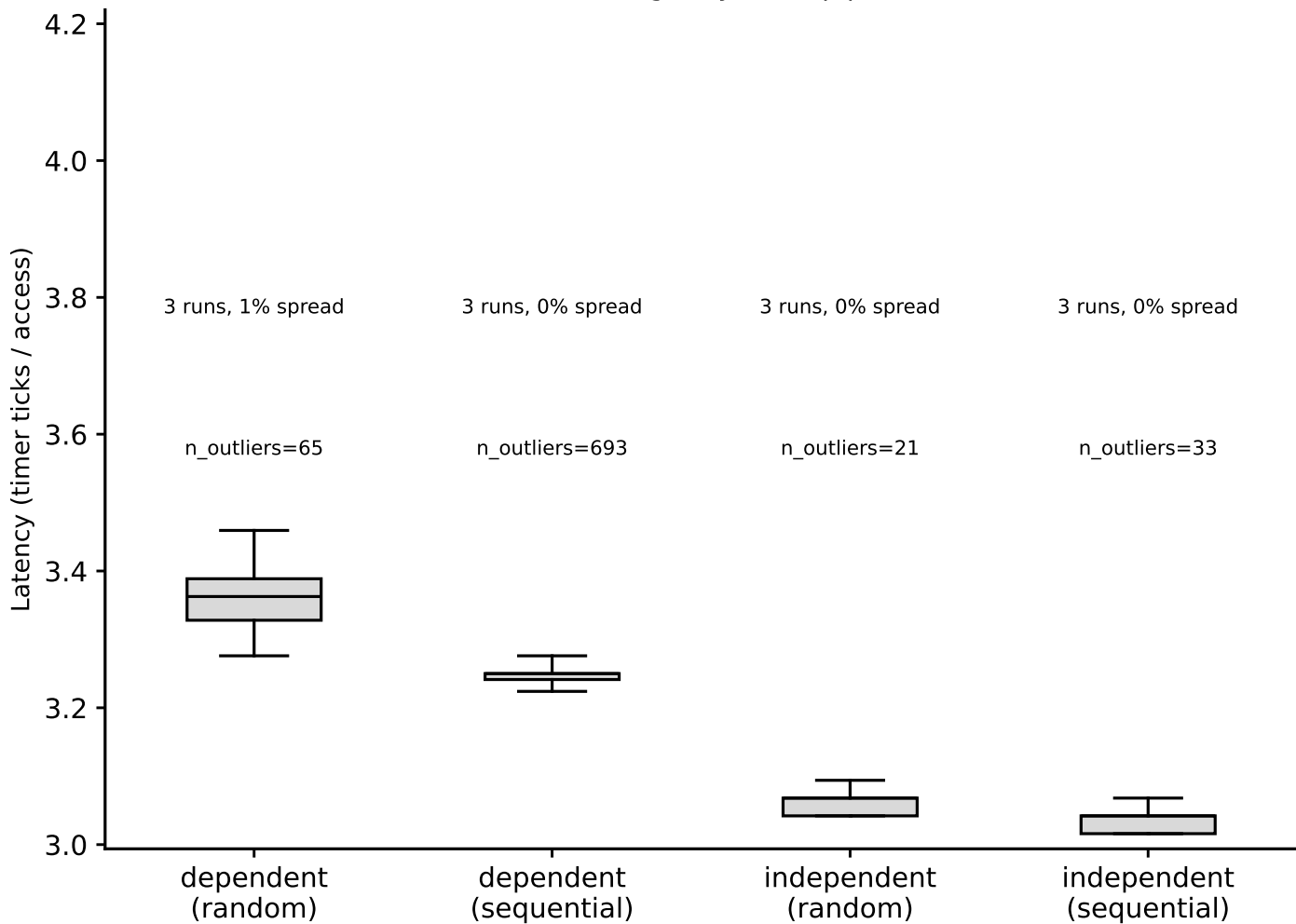
hazel_turin: hit-latency box plots, L1 (footprint=48 KiB) (Phase I timing-only, auto pipeline)
