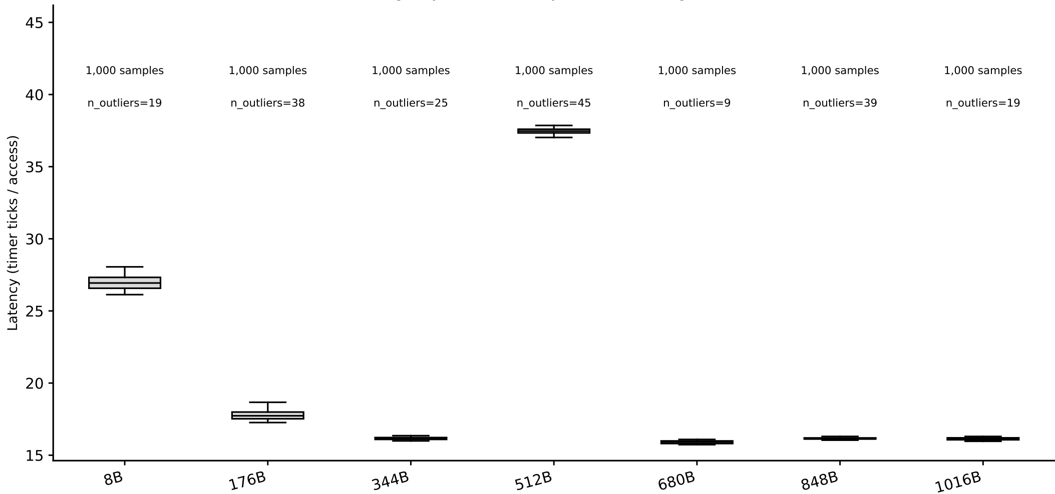
hazel_turin: line-size box plots, random pattern (whiskers = p5/p95) (Phase I timing-only, level boundary=1048576B, single-curve method)
