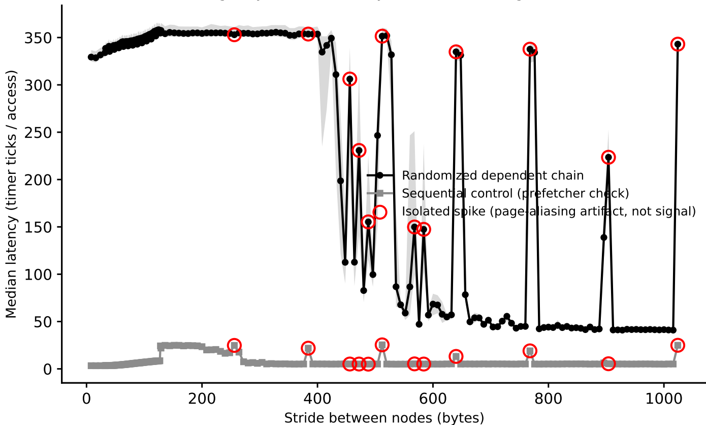
hazel_turin: line-size sweep (dependent pointer chase), footprint=64 MiB (Phase I timing-only, level boundary=33554432B, single-curve method)
