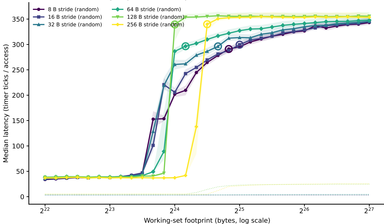
hazel_turin: line-size family of curves (dependent pointer chase) (Phase I timing-only, level boundary=33554432B window=[4194304,134217728])
