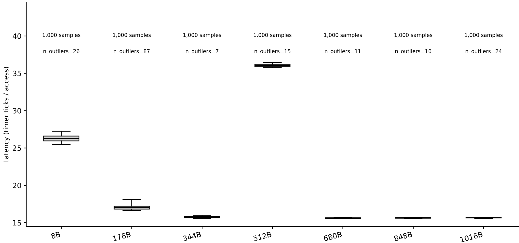
hazel_turin/line_size_rerun: line-size box plots, random pattern (whiskers = p5/p95) (Phase I timing-only, level boundary=1048576B, single-curve method)
