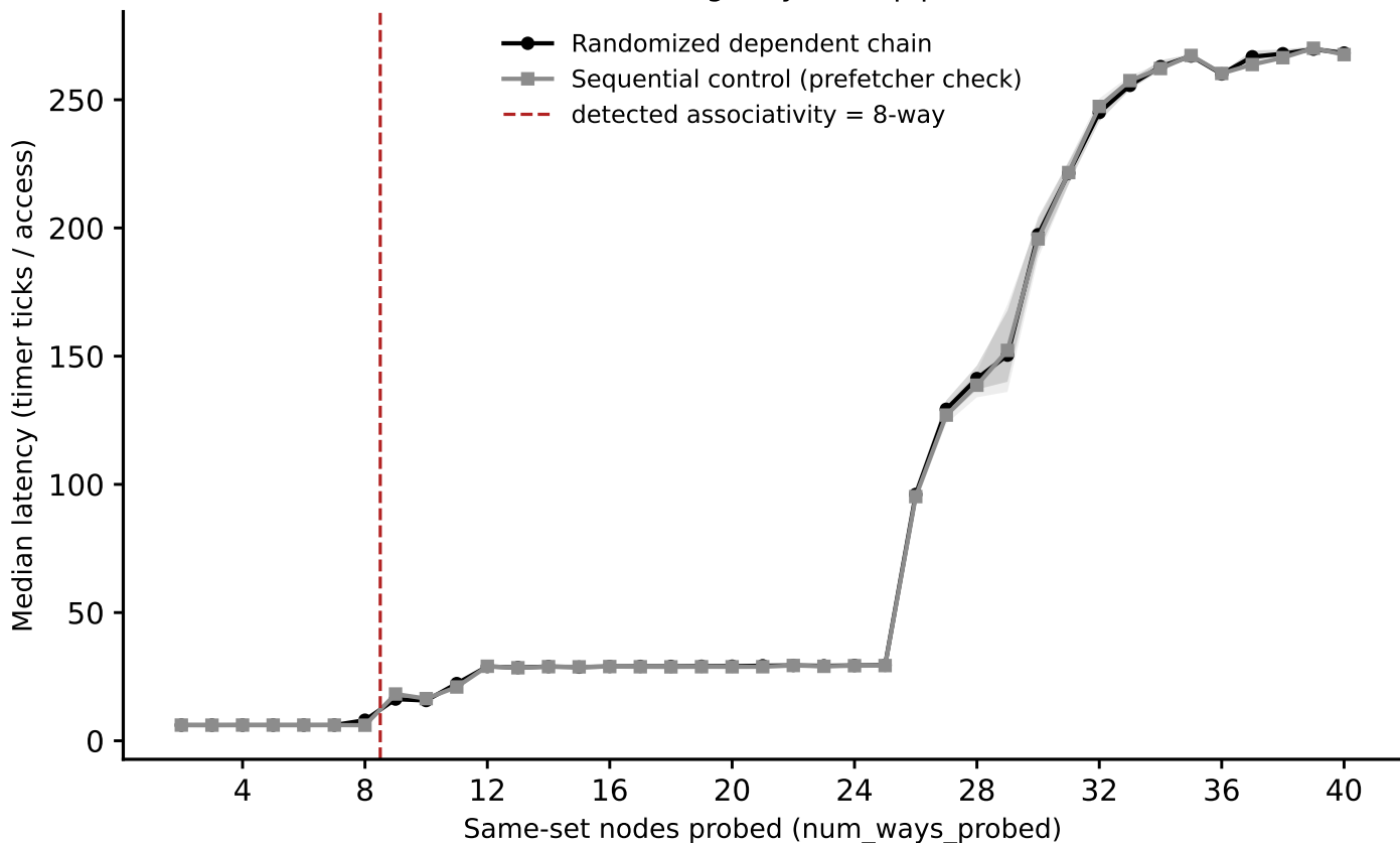
skylark: associativity sweep, L3_LLC (stride=8 MiB) (Phase I timing-only, auto pipeline)
