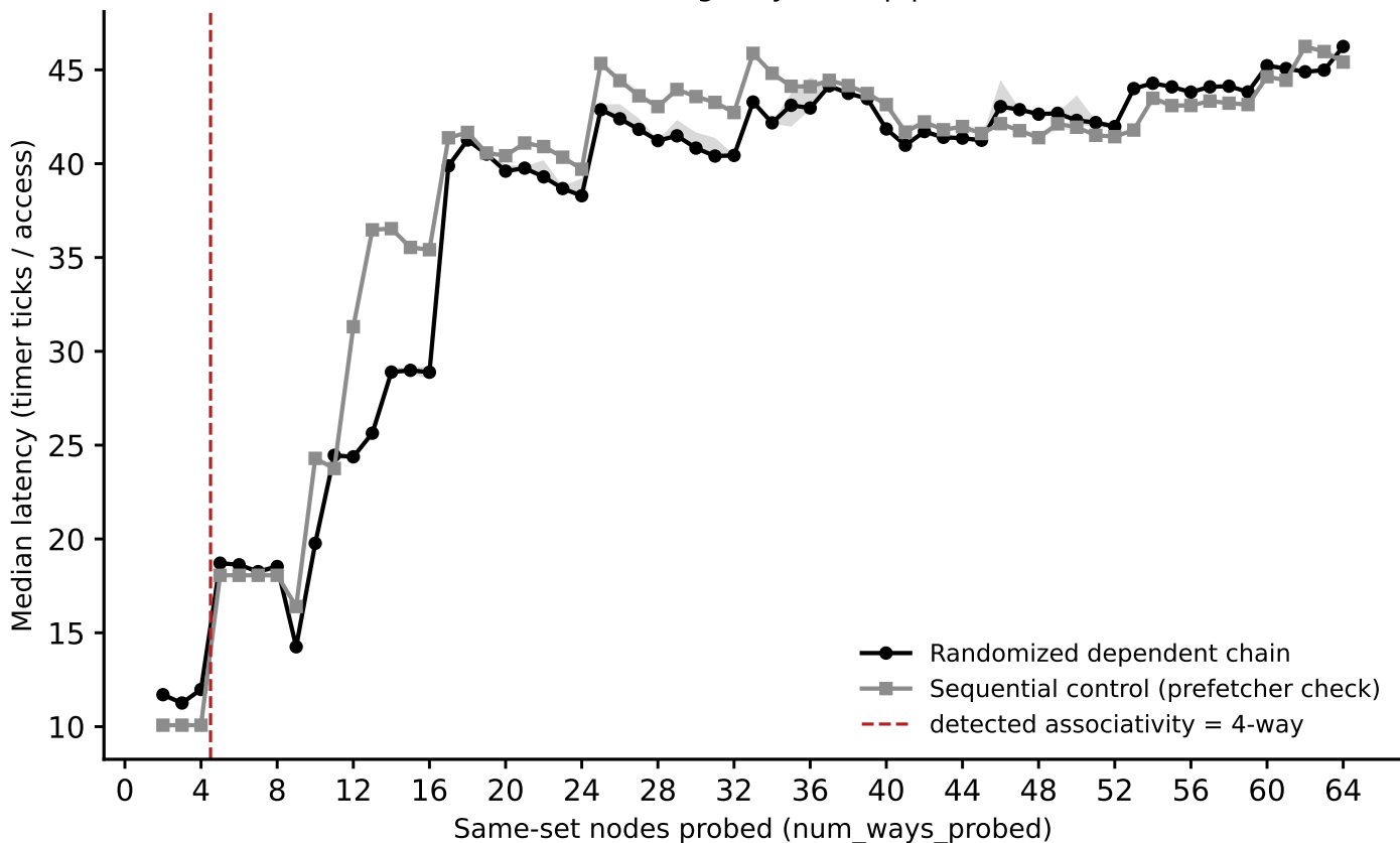
sunbird: associativity sweep, L2_256KiB_candidate (stride=256 KiB) (Phase I timing-only, auto pipeline)
