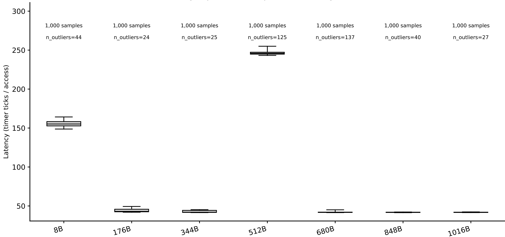
hazel_haswell: line-size box plots, random pattern (whiskers = p5/p95) (Phase I timing-only, level boundary=25165824B, single-curve method)
