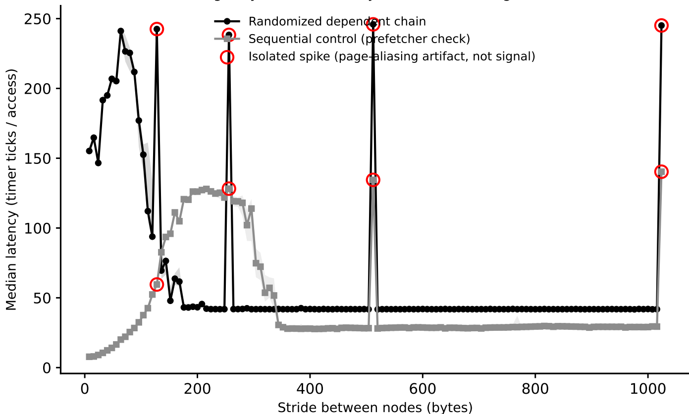
hazel_haswell: line-size sweep (dependent pointer chase), footprint=48 MiB (Phase I timing-only, level boundary=25165824B, single-curve method)
