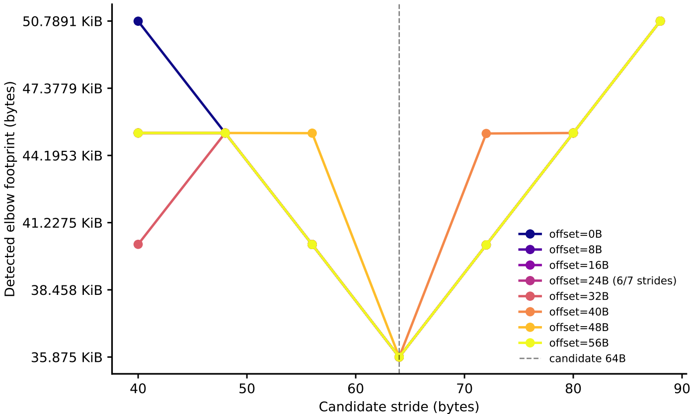
hazel_haswell: line-size elbow vs. stride, by node-0 offset (Phase I timing-only, level boundary=32768B, step-4 alignment refinement)
