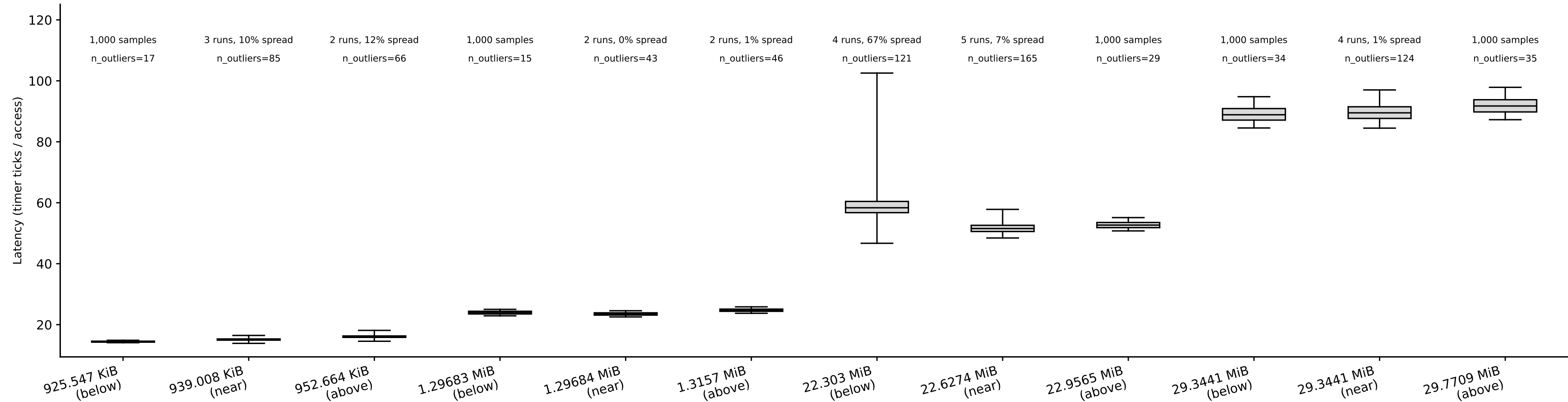
hazel_skylake: capacity box plots, random pattern (whiskers = p5/p95) (Phase I timing-only, auto pipeline) tested boundaries: 939.008 KiB, 1.29684 MiB, 22.6274 MiB, 29.3441 MiB
