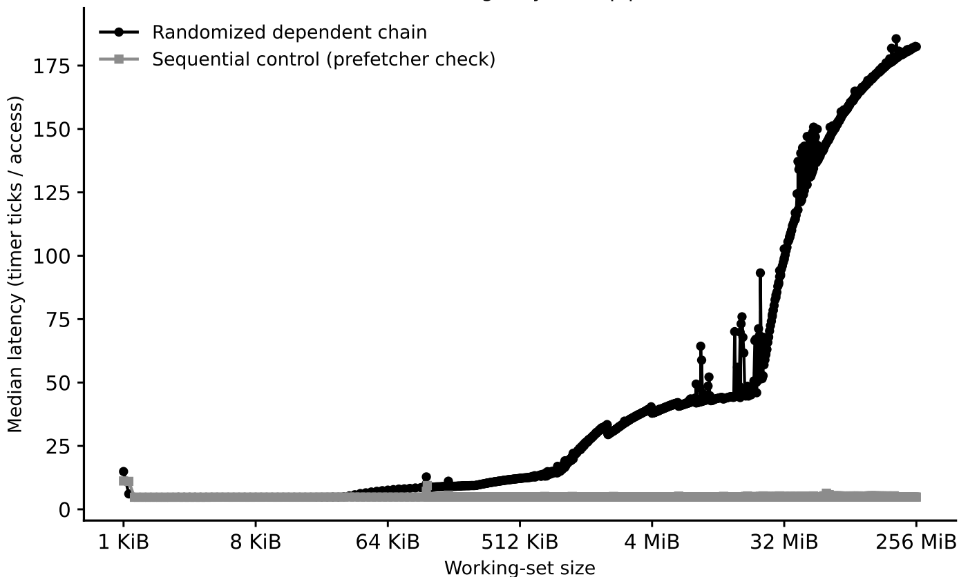
hazel_skylake: capacity sweep (dependent pointer chase) (Phase I timing-only, auto pipeline)
