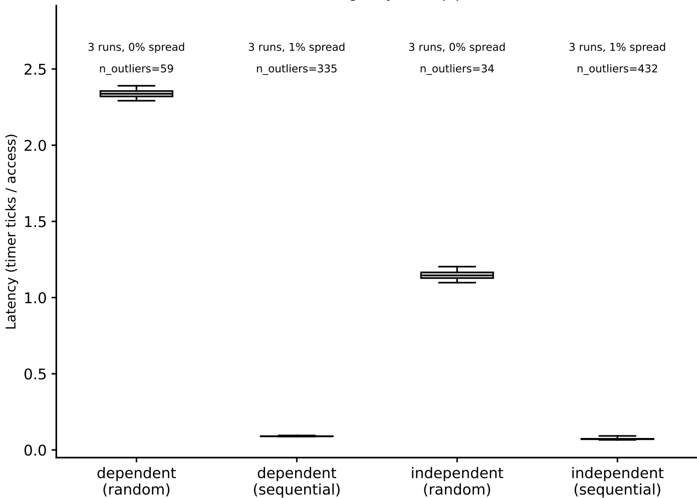
thunderbird: hit-latency box plots, DRAM (footprint=512 MiB) (Phase I timing-only, auto pipeline)
