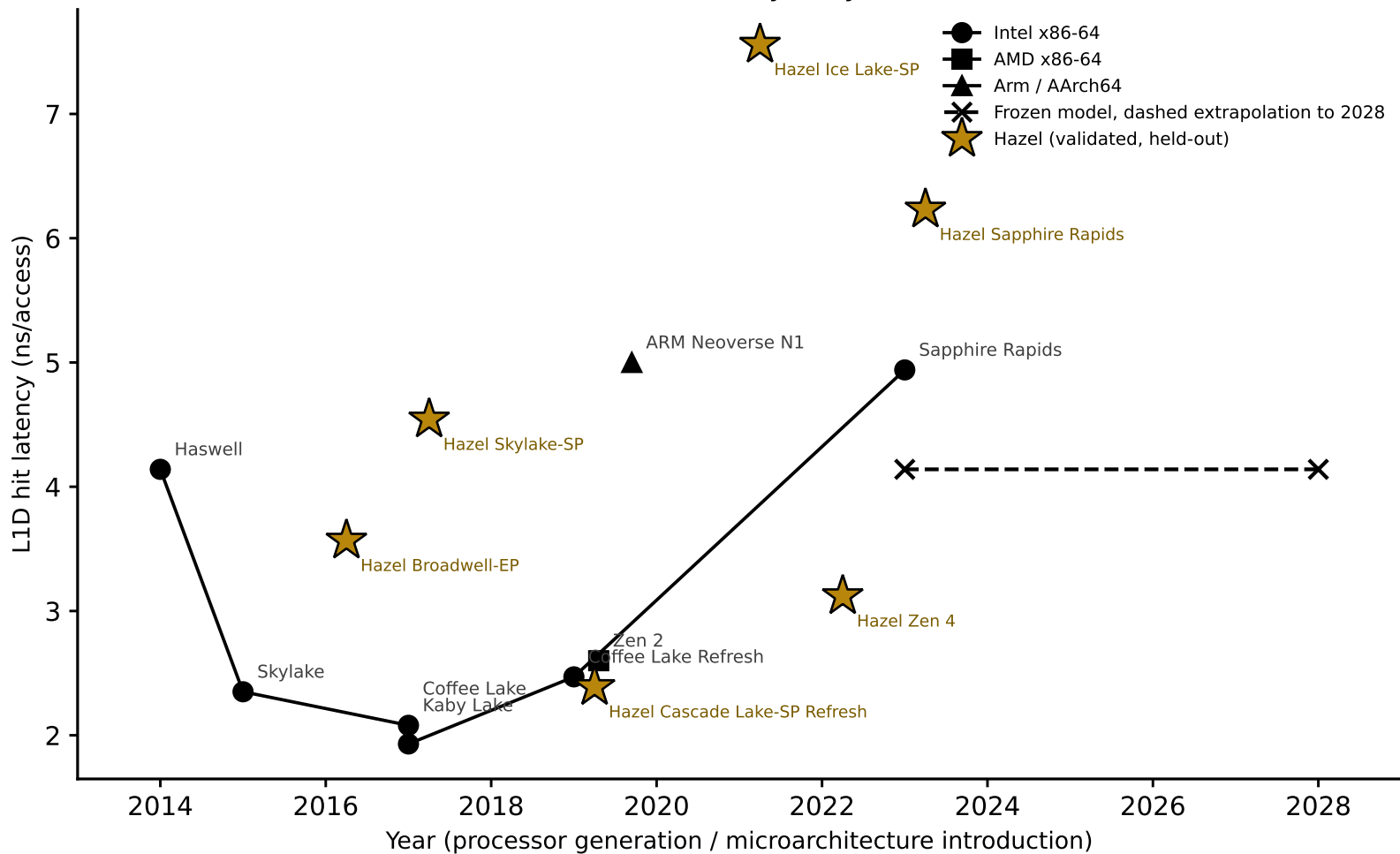
L1D hit latency vs. year
