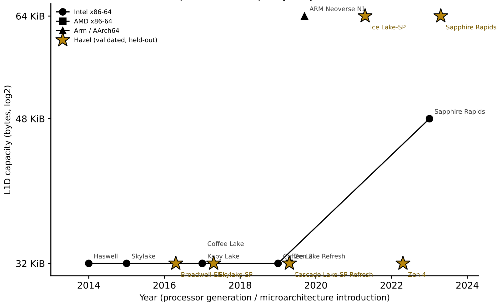
Final combined comparison: L1D capacity vs. year (lab + validated Hazel)
