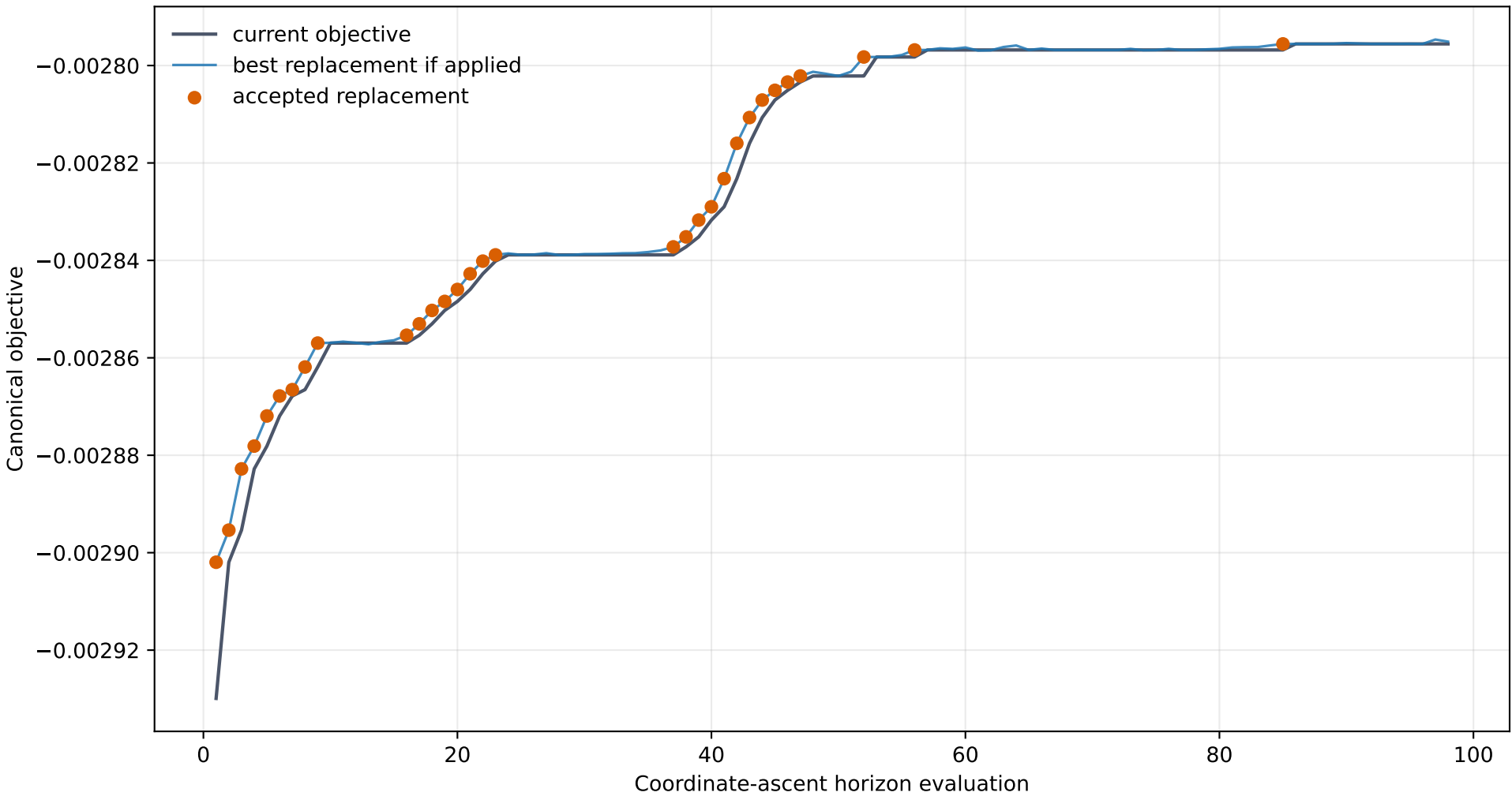
Coordinate polish objective at each potential replacement
