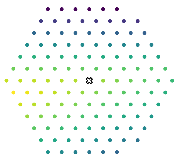
After smoothing, 20 years center=(0.26, 0.36, 0.38)
