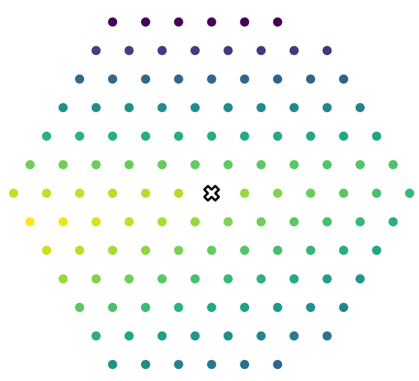
Before smoothing, 20 years center=(0.26, 0.36, 0.38)
