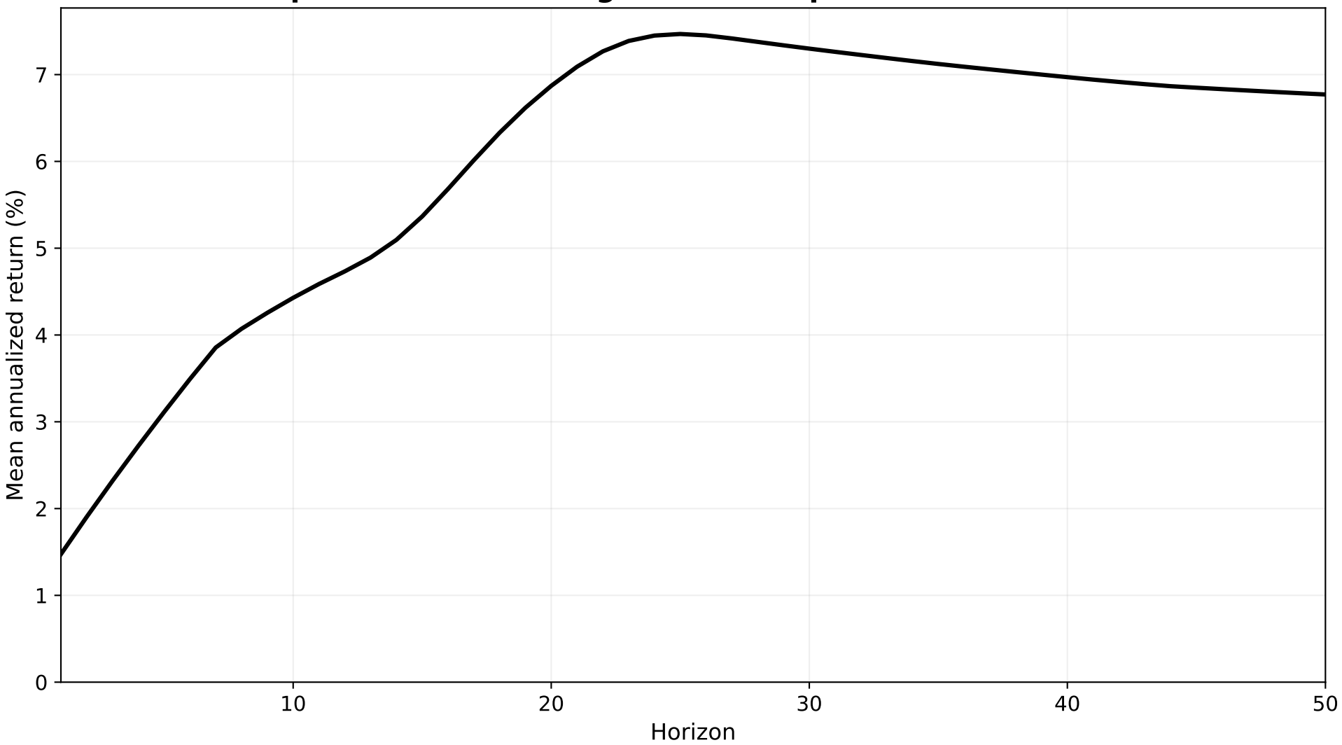
Expected Return Along the Stable q02 Path: Since 1927
