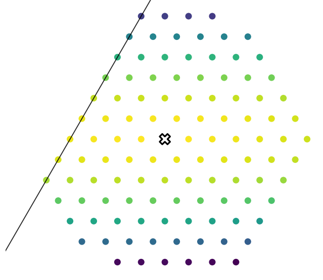
Before smoothing, 50 years center=(0.56, 0.36, 0.08)
