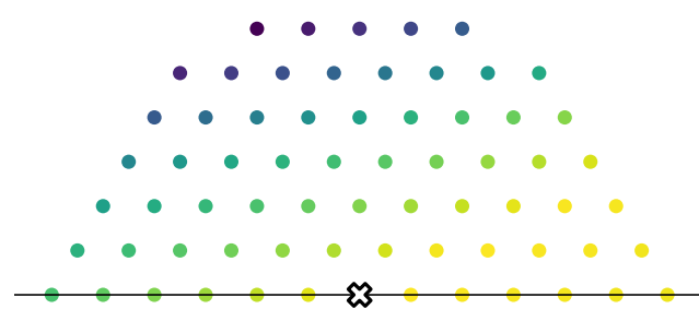
After smoothing, 1 years center=(0.00, 0.24, 0.76)
