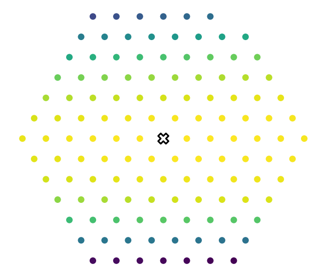
Before smoothing, 20 years center=(0.26, 0.68, 0.06)
