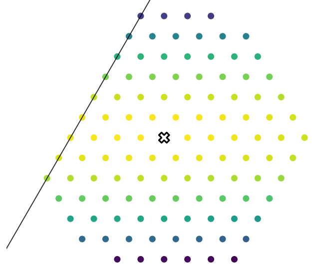
After smoothing, 50 years center=(0.56, 0.36, 0.08)
