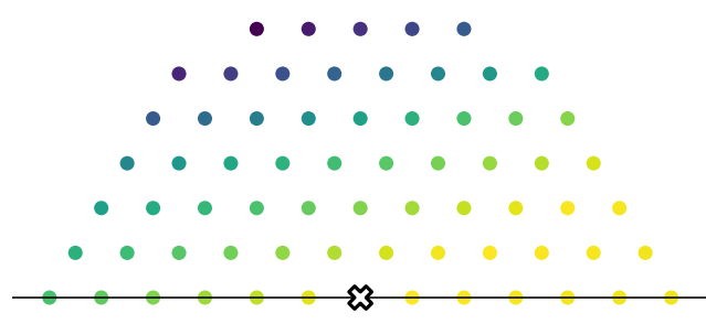
Before smoothing, 1 years center=(0.00, 0.24, 0.76)
