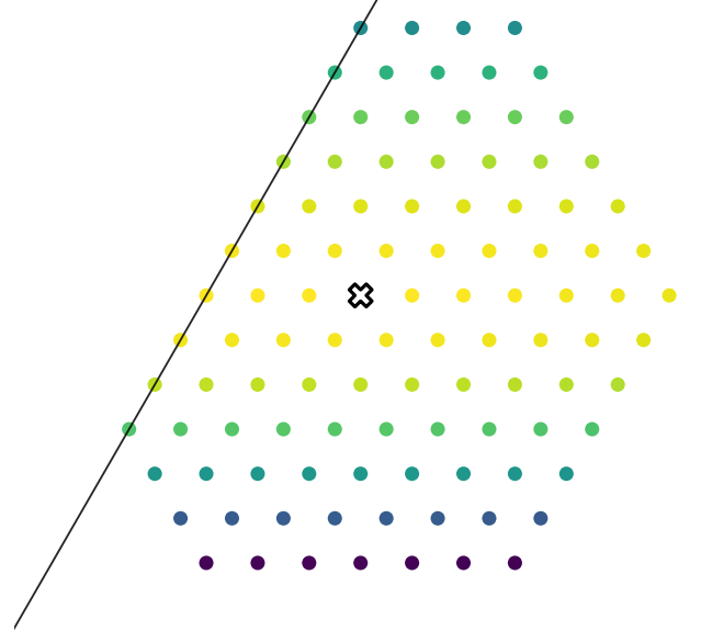
After smoothing, 50 years center=(0.56, 0.36, 0.08)
