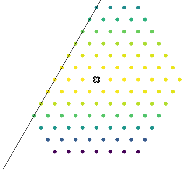
Before smoothing, 50 years center=(0.56, 0.36, 0.08)
