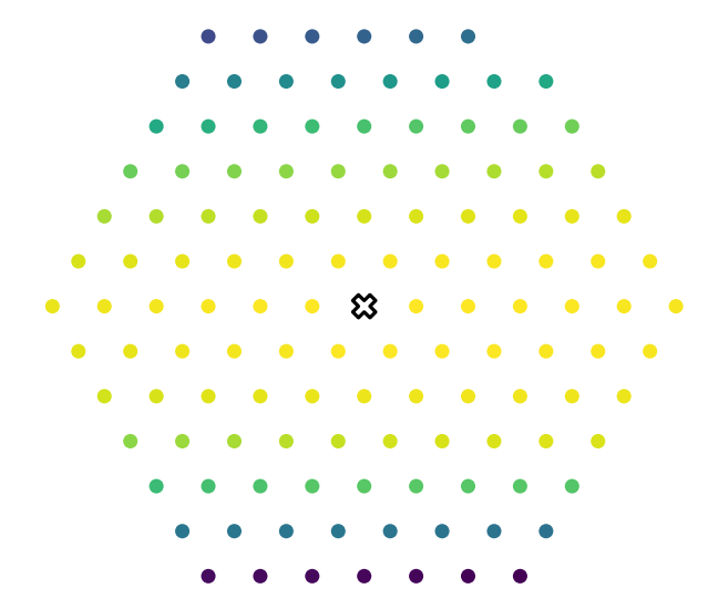
After smoothing, 20 years center=(0.26, 0.68, 0.06)
