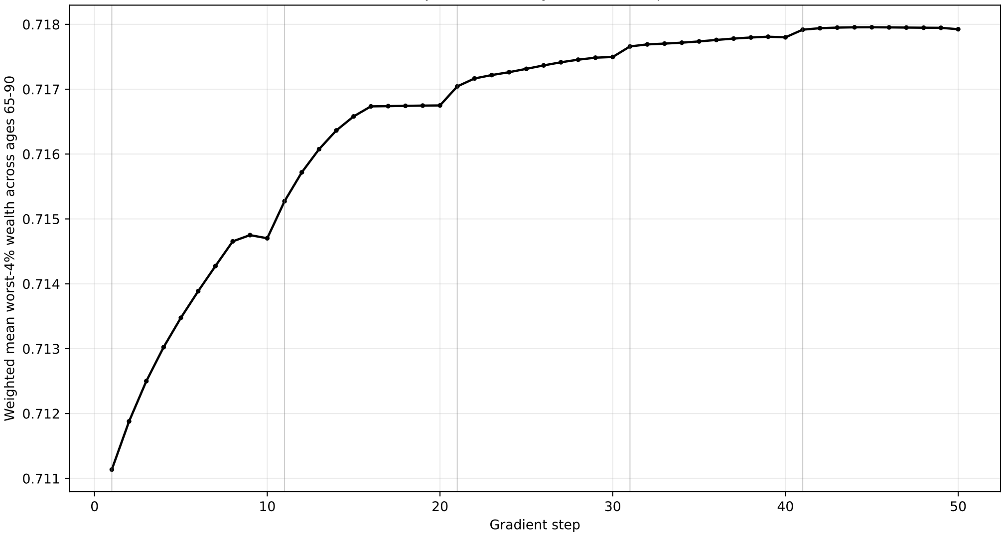
Objective at Every Gradient Step
