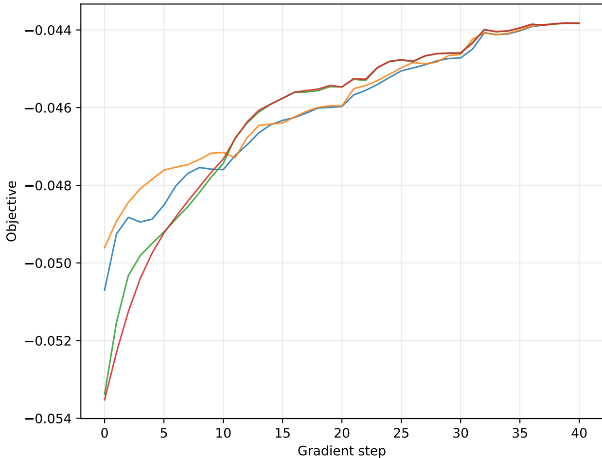
Canonical objective with exact horizon 1
