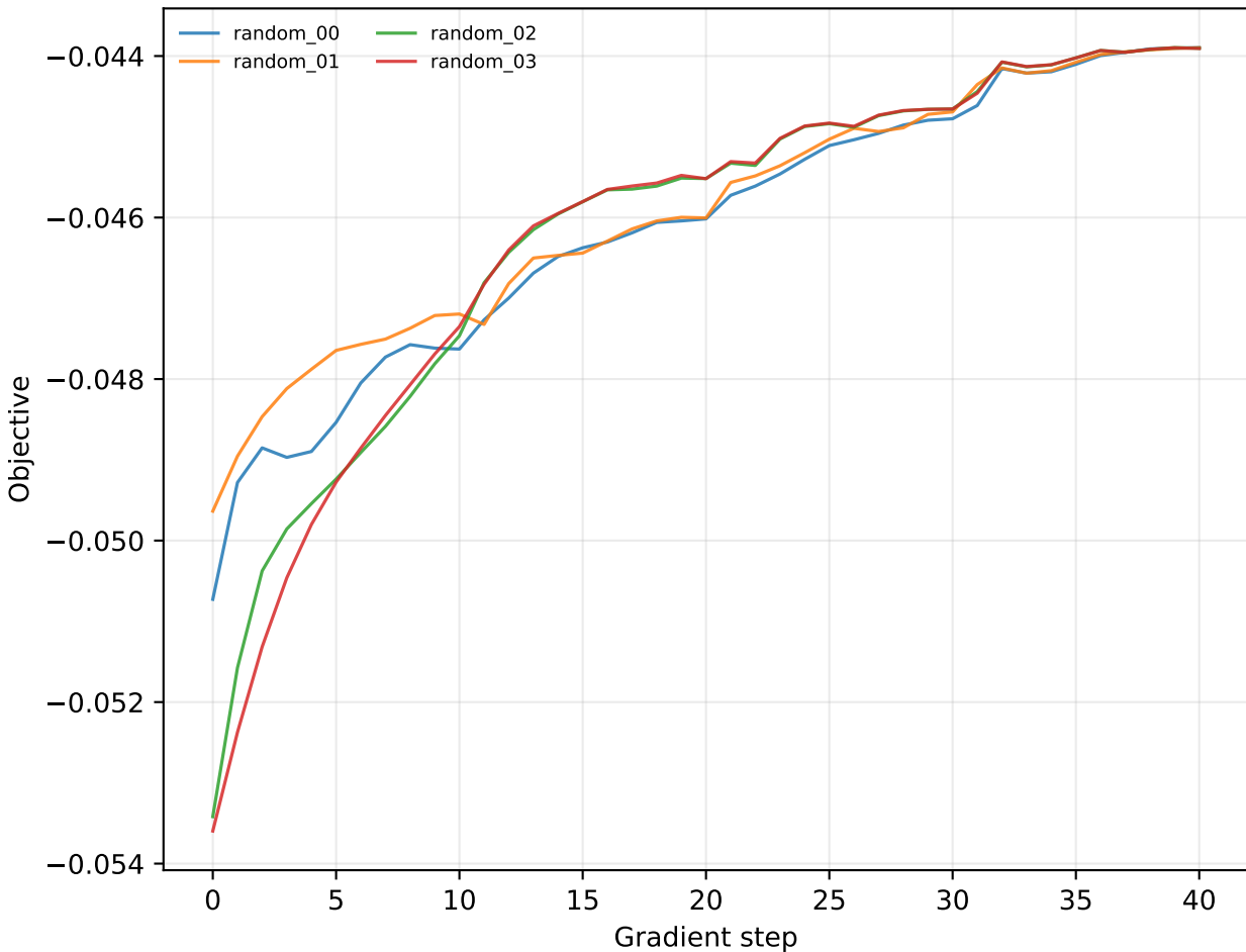
Regularized optimization objective
