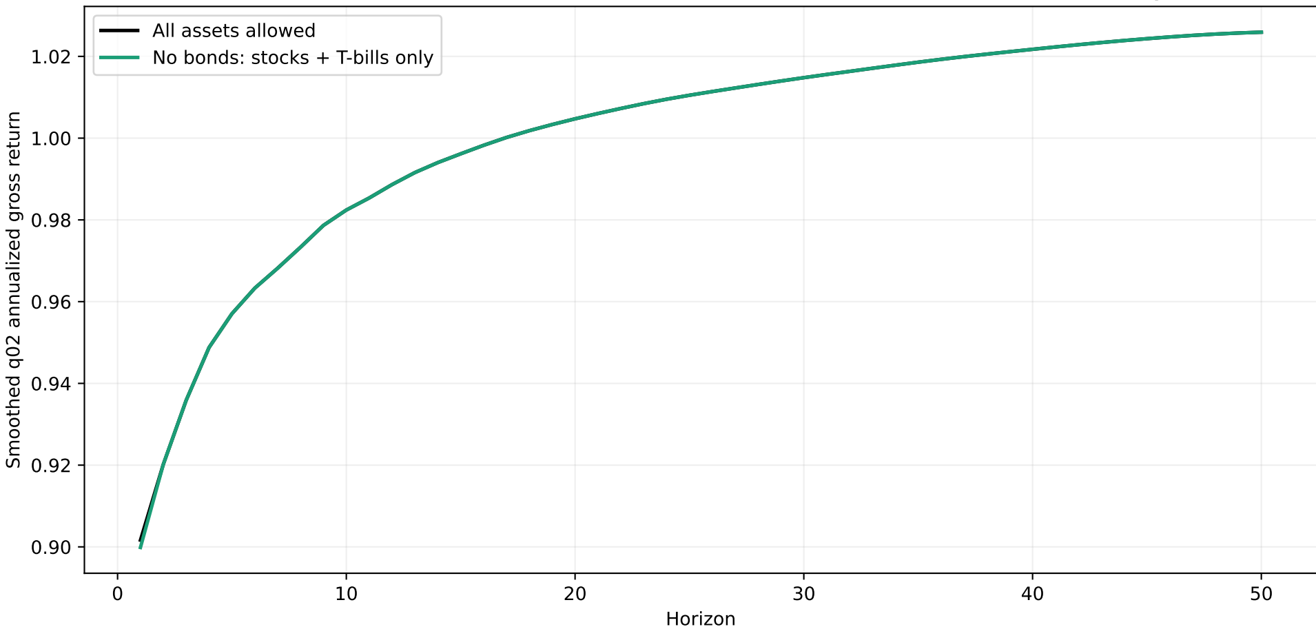
Best Smoothed q02 Annualized Return With vs Without Bonds: Full History
