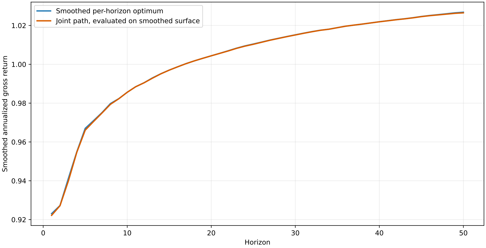
Smoothed q02 Return Cost of Joint Path Optimization: Since 1927 convex Gaussian smoothing with horizon bandwidth=0.7 years, portfolio bandwidth=0.05; raw horizon 1 a
