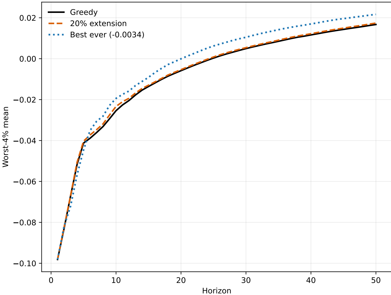
Glide Path Worst-4% Score
