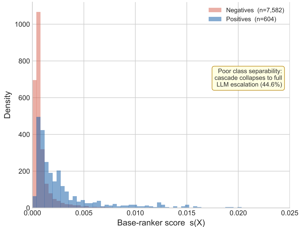
CD011975 — Score distribution
