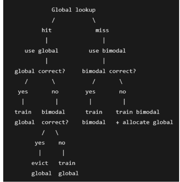
Figure 4: chatGPT generated diagram describing the table updating policy. 'train' corresponds to updating the 2-bit counter, and 'evict' corresponds to replacing the tag in the global table.
