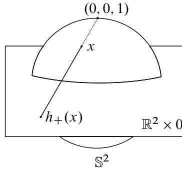
Figure 3: Stereographic projection
