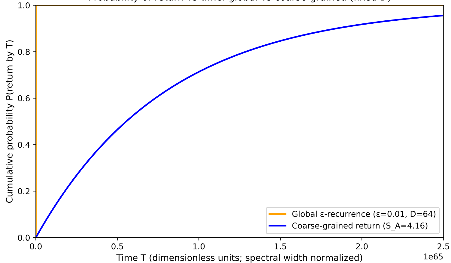
Probability of return vs time: global vs coarse-grained (fixed D)
