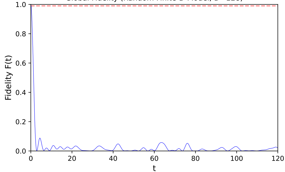
Global Fidelity (Random Finite-D Model, D=128 )
