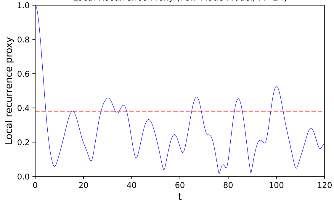
Local Recurrence Proxy (Few-Mode Model, M=24 )
