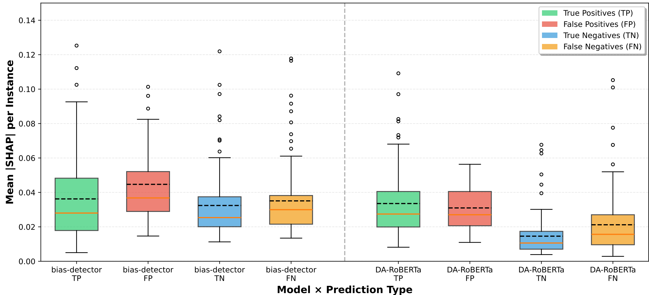
SHAP Magnitude Distributions by Prediction Type (BABE)
