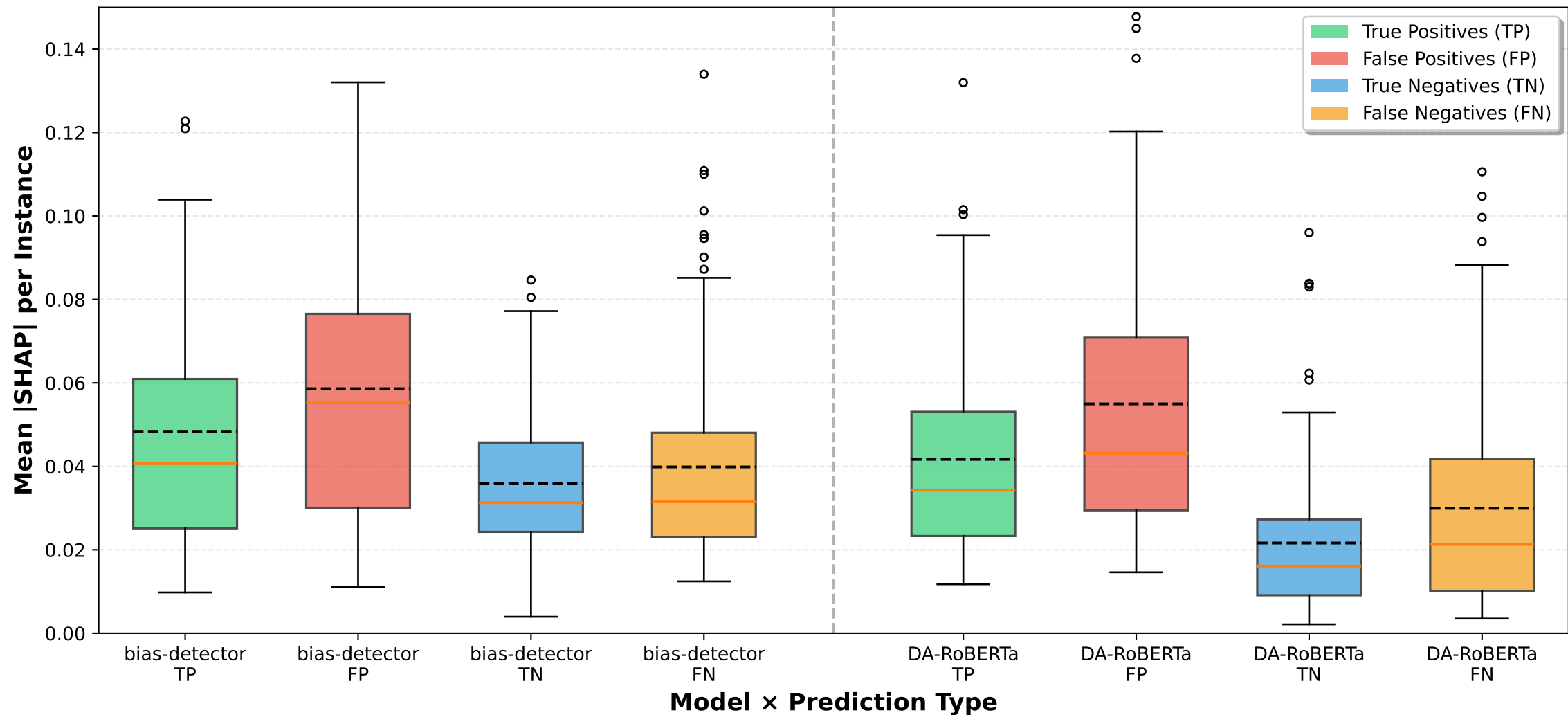
SHAP Magnitude Distributions by Prediction Type (BASIL)
