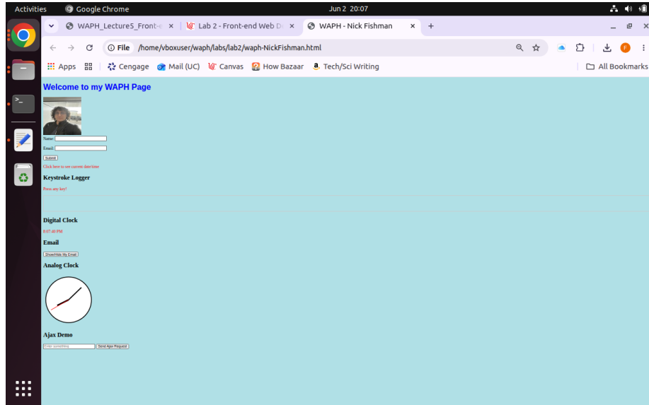
Figure 5: CSS Demo
