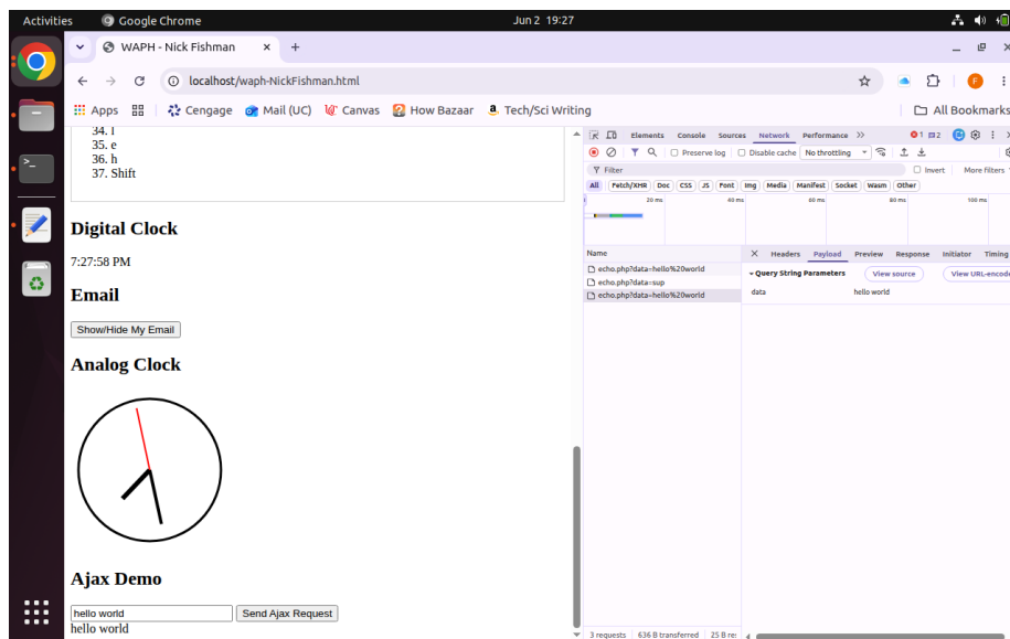
Figure 4: Ajax Demo (Payload)
