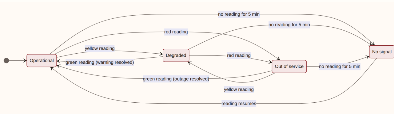
Figure 3.2 · Station states. The four words used everywhere. "No signal" is not a fault; it means the station's status is unknown, and that time is left out of every rate.
