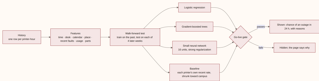
Figure 4.1 · Train, test, gate. Recent history counts more (weight halves every 21 days). The model retraines nightly; every prediction is logged so its track record can be checked later.
