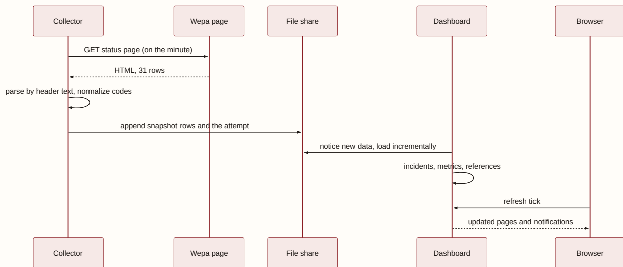
Figure 6.2 • The one-minute cycle. Once a day the collector also compacts finished days, refreshes campus data and weather, retrains the risk model, checks for vulnerabilities and sends queued feature requests.
