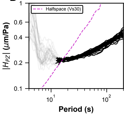
D Transfer Function: 544A
