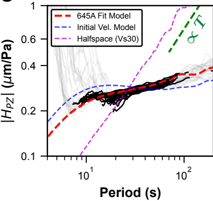
C Transfer Function: 645A
