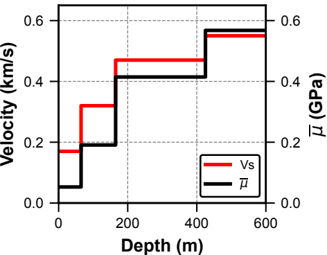
A Elastic Structure
