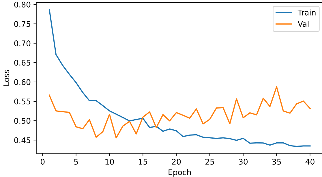
Loss curves
