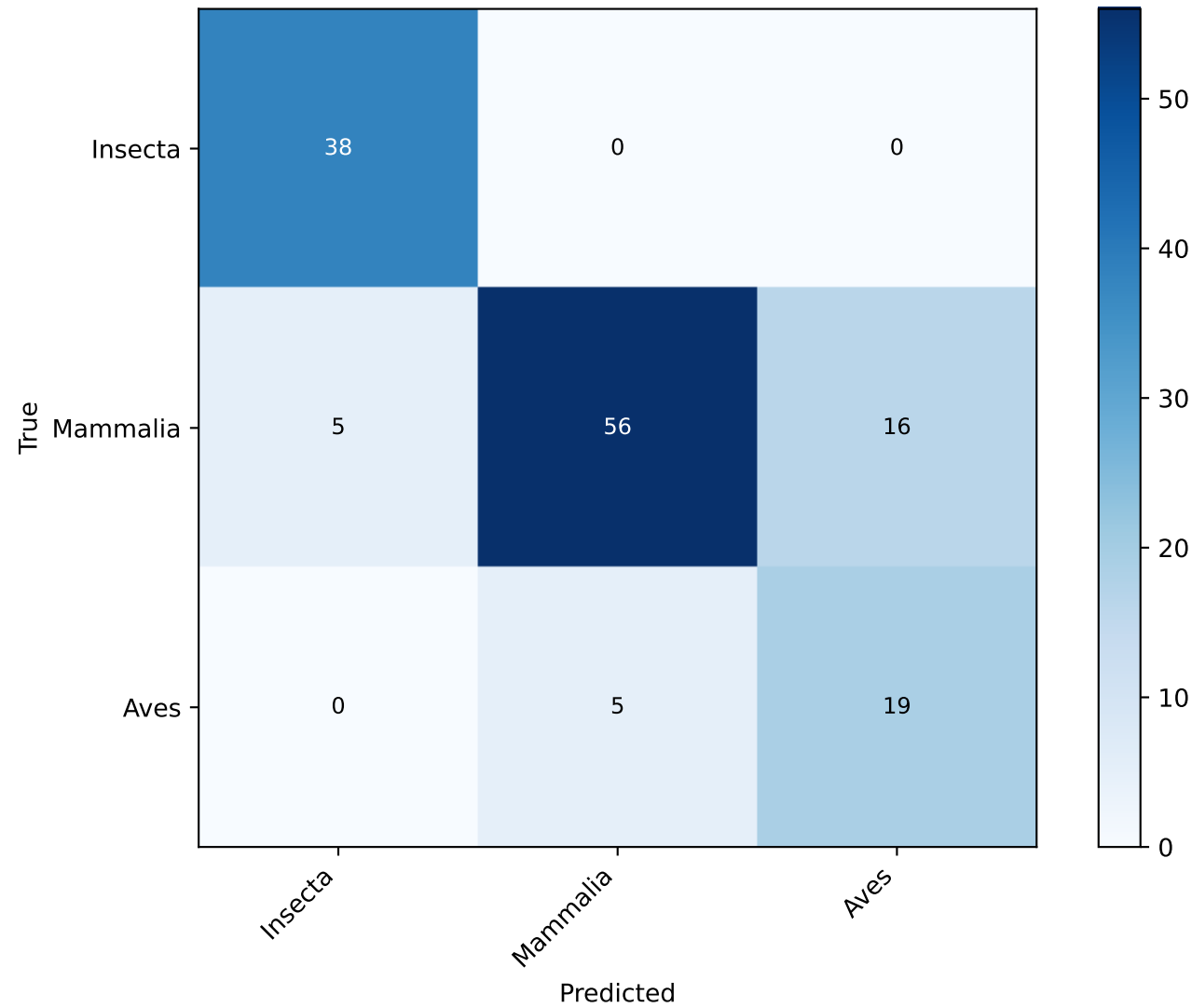
Confusion matrix — Raw counts
