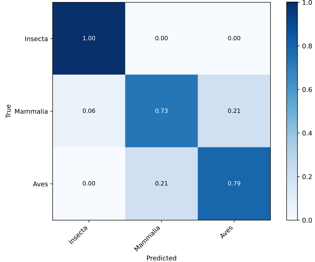
Confusion matrix — Row-normalised (recall)
