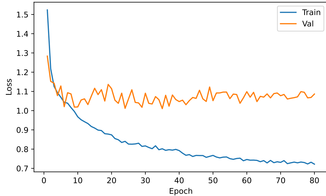
Loss curves
