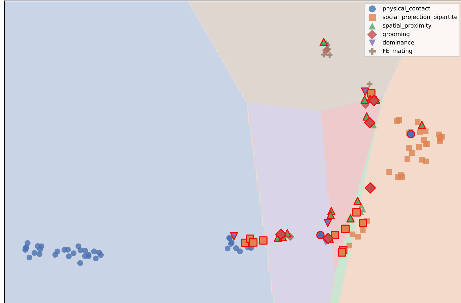
GCN decision regions in UMAP space
