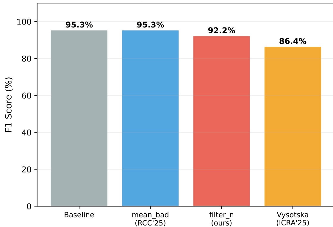
Closed-Set (all queries have a match)
