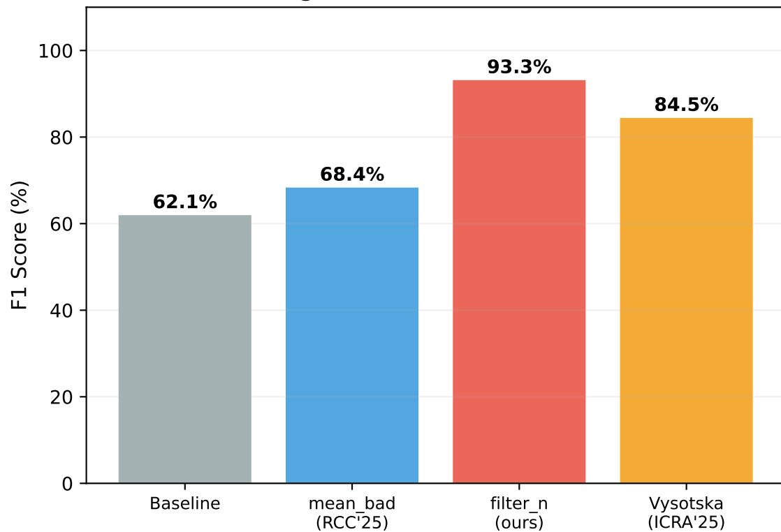
Open-Set (50% genuine + 50% distractors)
