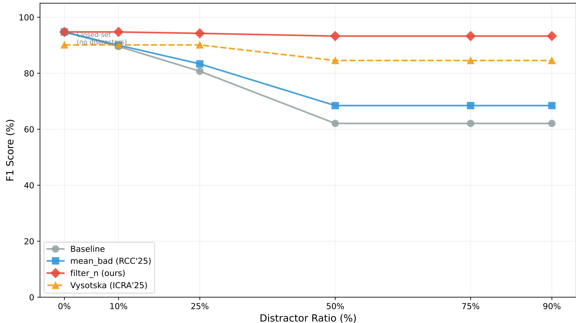
Robustness to Distractor Ratio: F1 Score as Unknown Queries Increase
