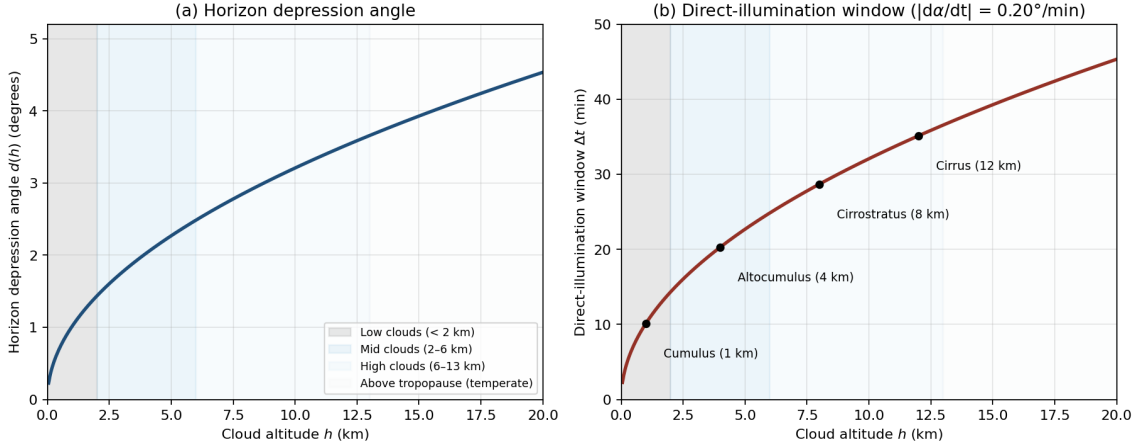
Figure 2: Cloud altitude controls illumination duration after sunset. Left: horizon depression angle d(h) = \arccos(R_\oplus/(R_\oplus + h)) as a function of cloud altitude h . Right: direct-illumination time window \Delta t(h) = 2d(h)/|d\alpha/dt| from apparent sunset, using a representative mid-latitude solar elevation rate |d\alpha/dt| = 0.20^\circ/\text{min} . Annotations show typical cloud-type altitudes. WMO three-tier altitude bands (low, mid, high) shaded in both panels.
