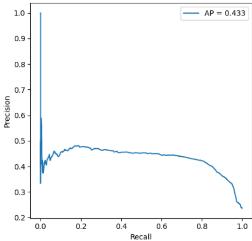
Precision-Recall Curve
