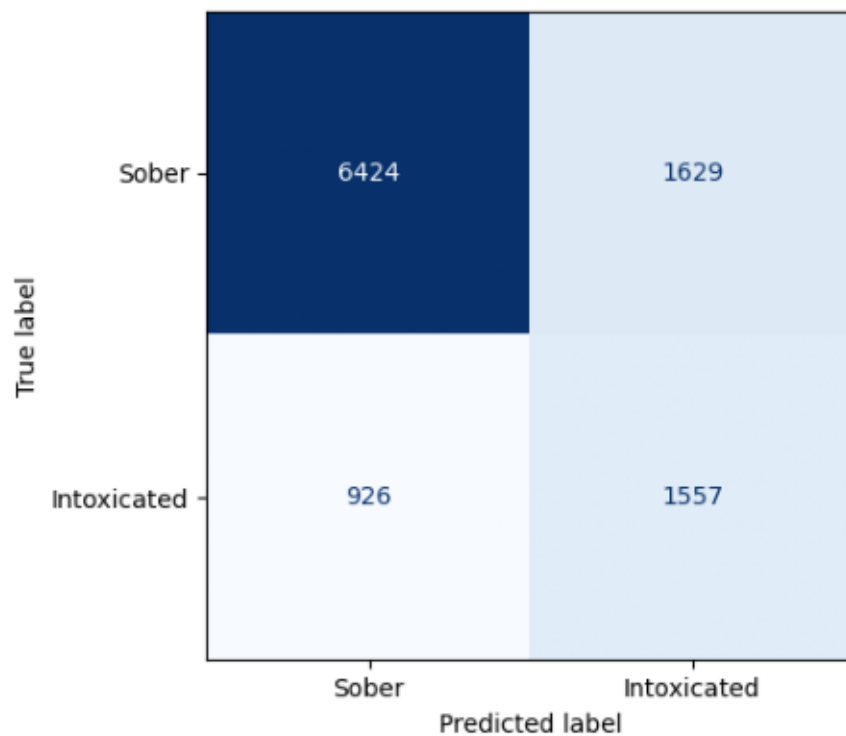
Confusion Matrix
