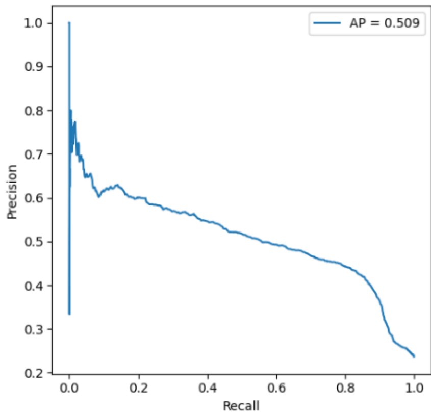
Precision-Recall Curve
